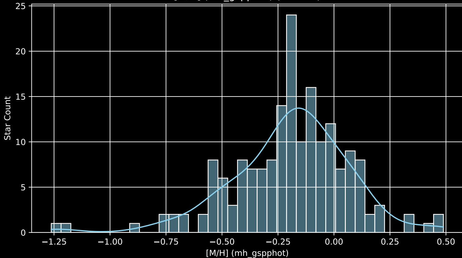
APOGEE DR17 Field: [CVZTILE_089+27_btx [M/H] (mh_gspphot) (n= 178)
