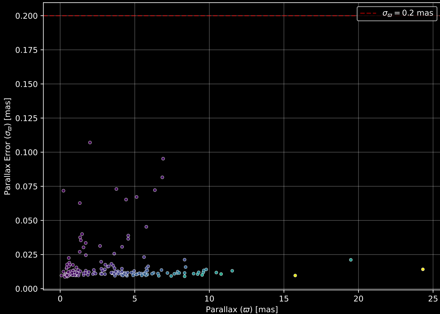
APOGEE DR17 Field: [CVZTILE_089+27_btx] Parallax Quality (n= 179)
