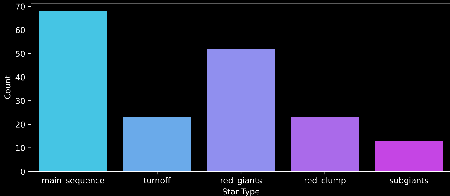
APOGEE DR17 Field: [CVZTILE_089+27_btx] Count plot of Star Type
