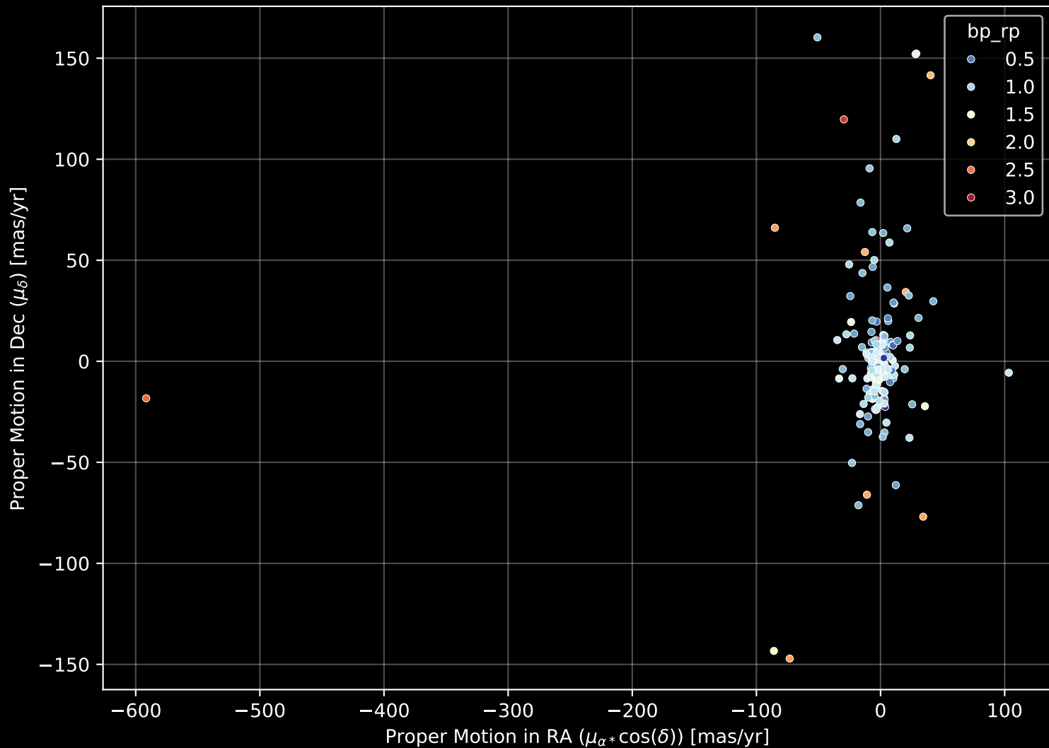
APOGEE DR17 Field: [CVZTILE_089+27_btx] Proper Motion Diagram (n= 179)
