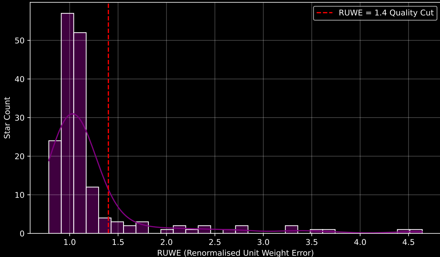
GAPOGEE DR17 Field [CVZTILE_089+27_btx] RUWE Distribution (n= 172)
